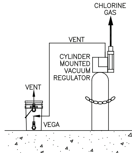
Typical Arrangement
